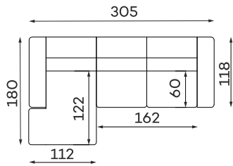
LUST SET 1 CORNER
