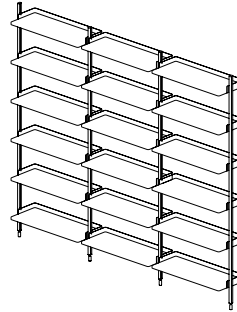
PIER SYSTEM | 103 WIDTH 242 CM | 95.25" DEPTH 31,5 CM | 12.50" HEIGHT 209 CM | 82.25"
