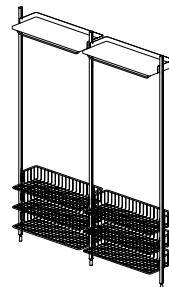
PIER SYSTEM | 1022 WIDTH 162 CM | 63.75" DEPTH 31,5 CM | 12.50" HEIGHT 209 CM | 82.25"
